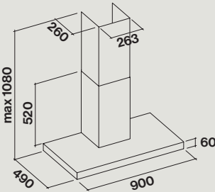
Plane Green Tech – 800 m³/h
