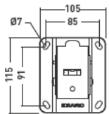
Platine murale
